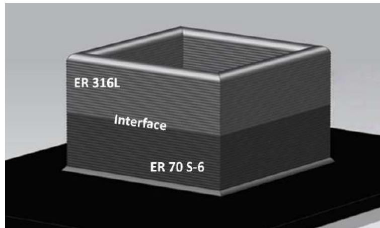
Figure 2. Schematic illustration of the deposited layers of the multi-material component.
