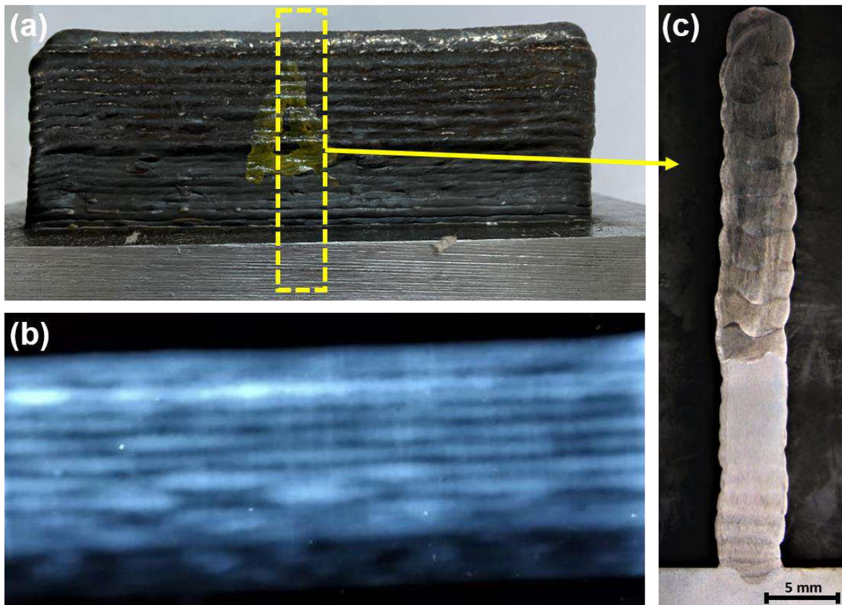
Figure 4. a) The front view, b) the X-ray result, and c) the macro-section of WAAM processed component.
