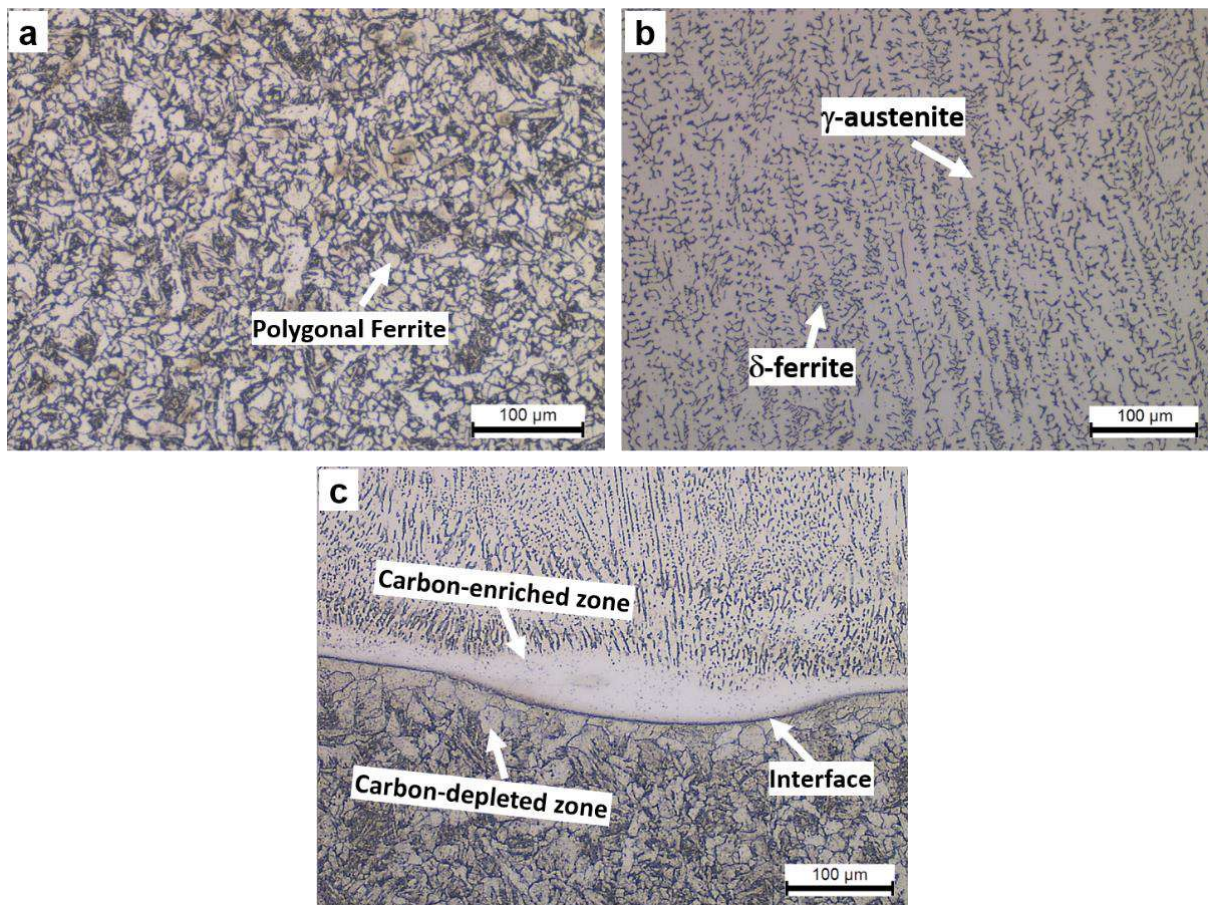
Figure 5. Micrographs of the deposited two layers with two different filler metals; a) ER 70 S-6 side, b) ER 316 L side, and c) interface.
