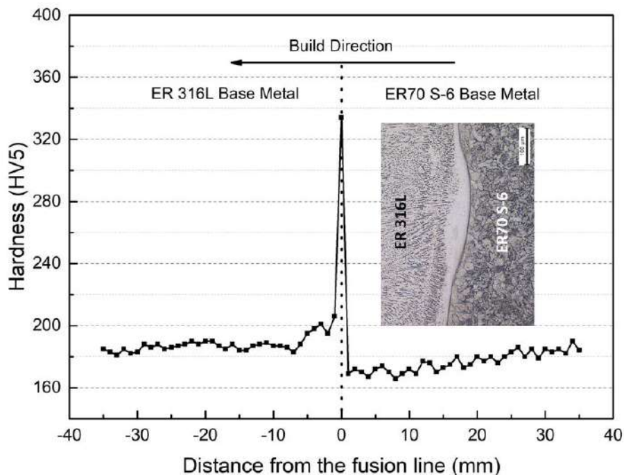
Figure 7. Vickers hardness test result of the as-deposited layers and interface.
