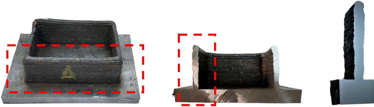
Figure 3. The final form of the WAAM processed as-built component and the specimen preparation process.
