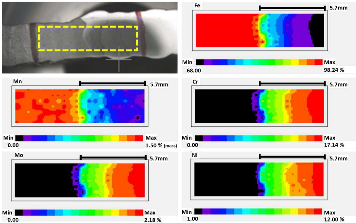
Figure 6. The elemental chemical composition mapping of the cross-sectional profiles of WAAM processed multi-layer sample.
